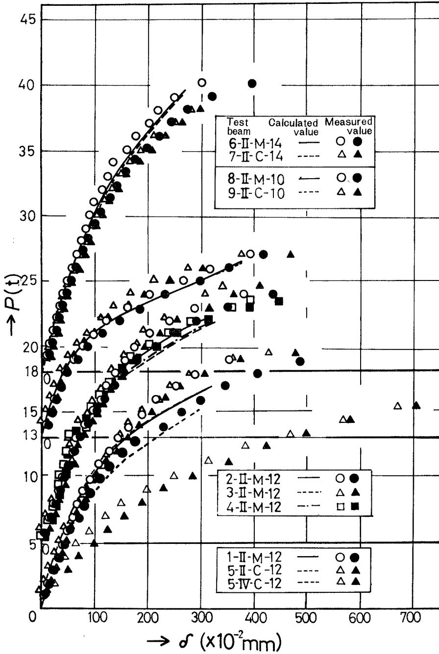
Fig.8 (b) Deflection
