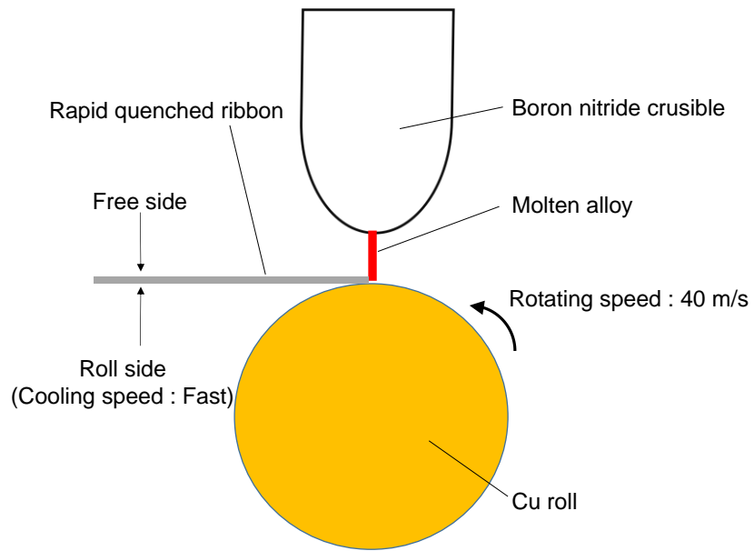
Figure S1. Schematic diagram of roll quenching method
