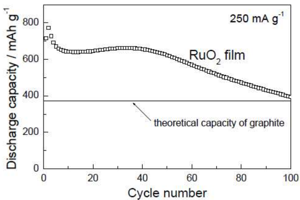
Fig. 1. Dependence of discharge capacity on cycle numbers for RuO 2 thick film electrode prepared by gas-deposition. The charge-discharge measurements were carried out in the electrolyte solution of PC containing LiClO 4 .
