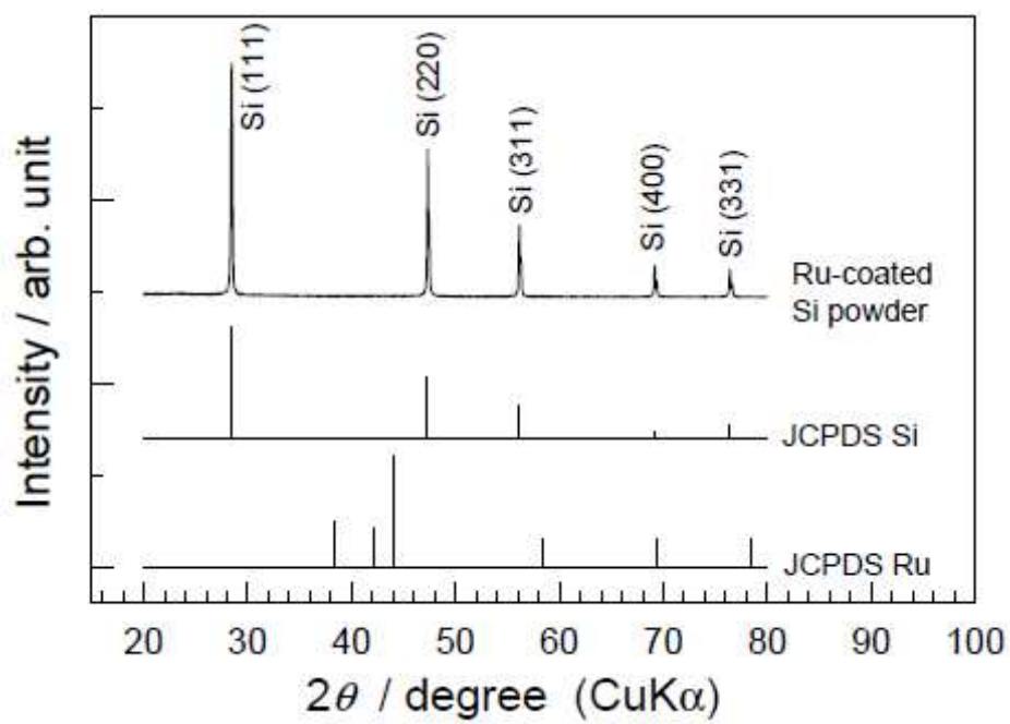
Fig. 6. XRD pattern of Ru-coated Si powder prepared by the ELD method.
