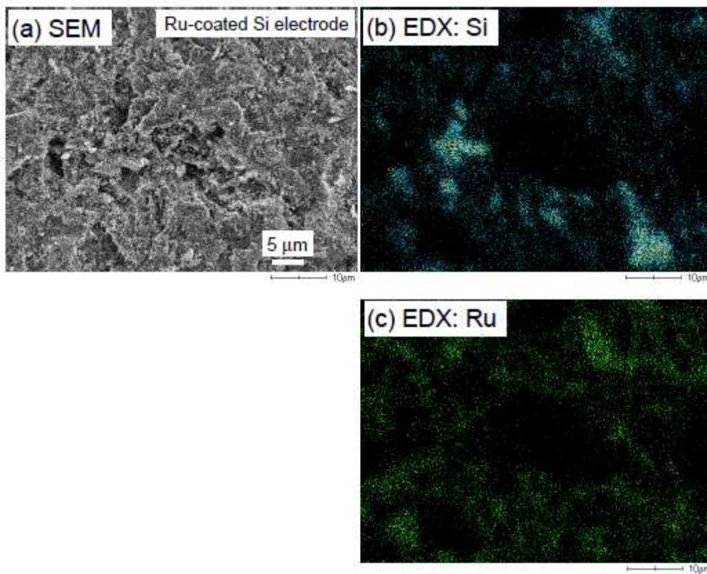
Fig. 8. (a) SEM image of the thick film electrode consisted of Ru-coated Si on the Cu substrate prepared by the gas-deposition. EDX results of element mapping for (b) Si and (c) Ru.
